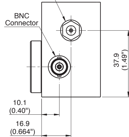
Power Supply Connector (On 7Z02506 Only)
